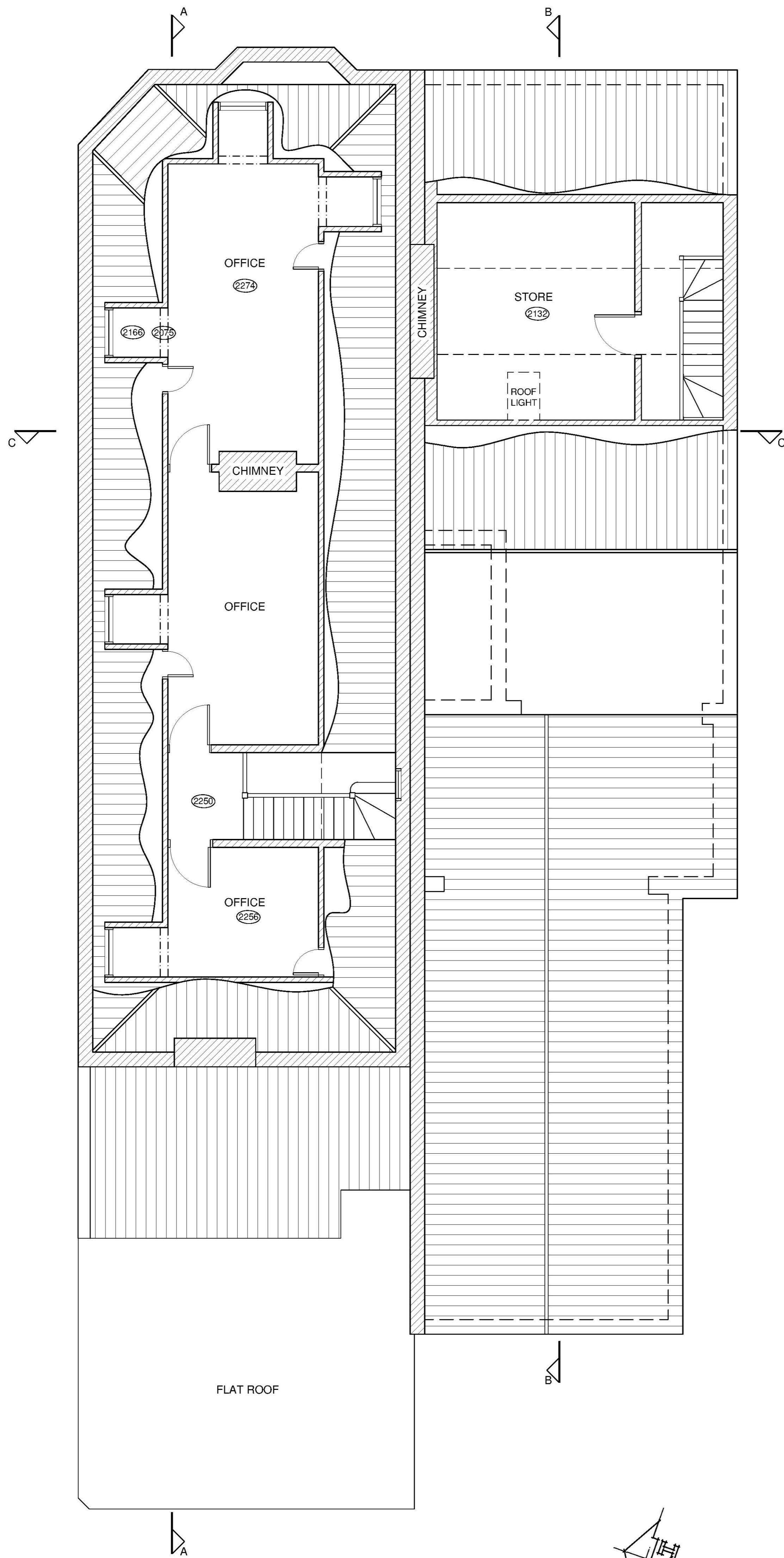
EXISTING THIRD FLOOR PLAN
